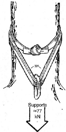
A Wrap 3-Pull 2 tie-off with webbing could yield anchor strength as high as 77kN (18,000 lbf) if the angles at the carabiner are kept less than 30°.
